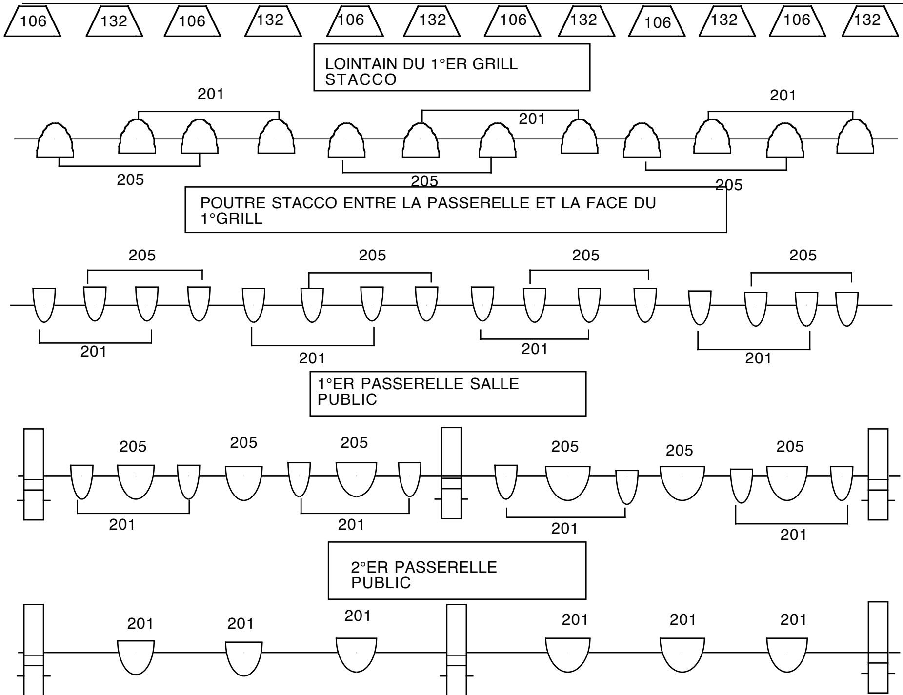
Plan lumière studio de concert BFM
